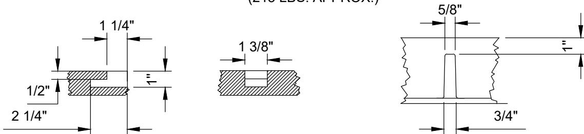
PICKHOLE DETAILS
