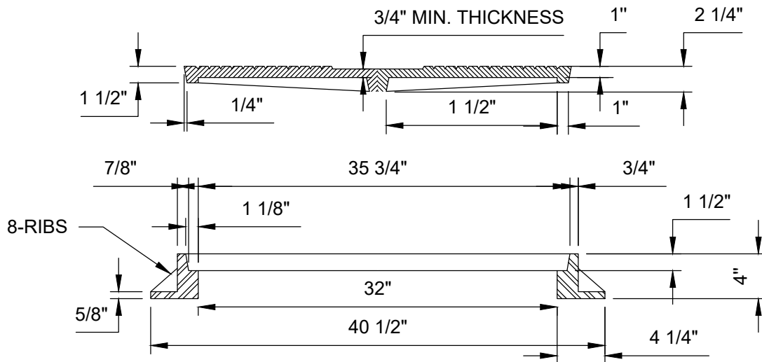
FRAME (215 LBS. APPROX.)
