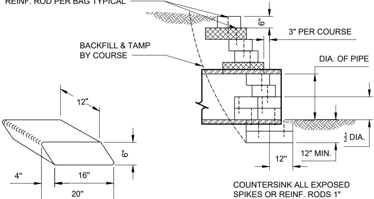
SECTION F-F
