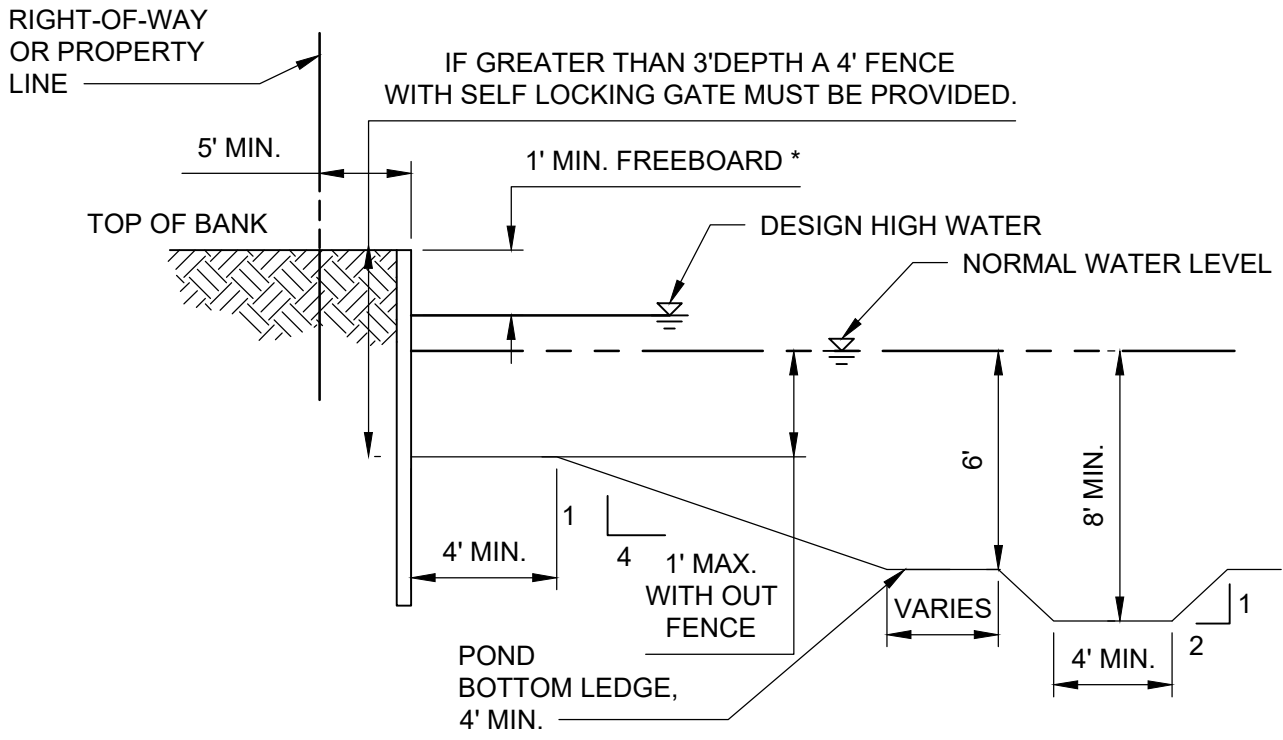
CASE 3 WET DETENTION POND
