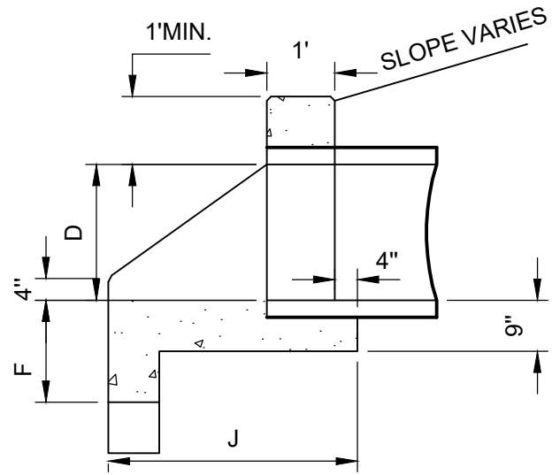
SECTION R-R
