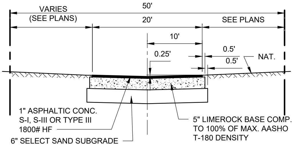
PRIVATE DRIVES ONLY TYPICAL CROSS SECTION
