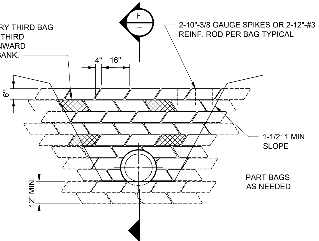
BAG DETAIL
