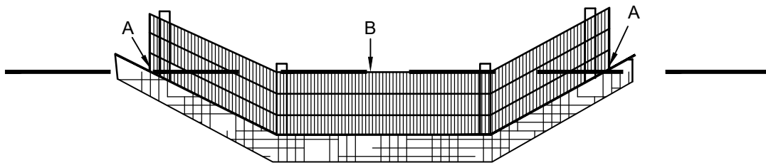
PROPER PLACEMENT OF BALE BARRIER IN DRAINAGE WAY
