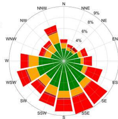
IFF 1 - eNose 6
